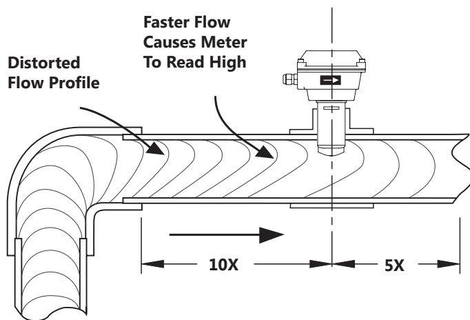
Distorted Flows
